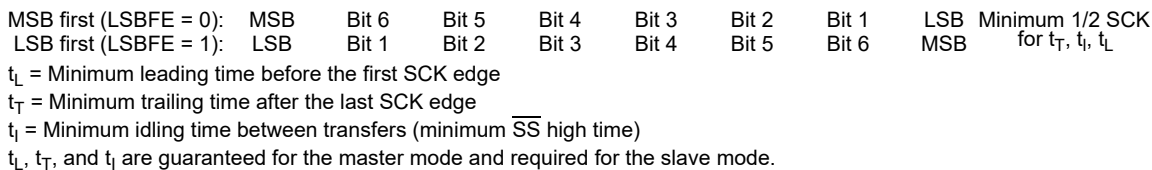
Figure 21-12. SPI Clock Format 0 (CPHA = 0), with 8-bit Transfer Width selected (XFRW = 0)
