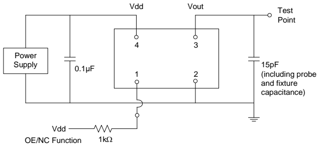
Figure 2. Test Circuit [6]
