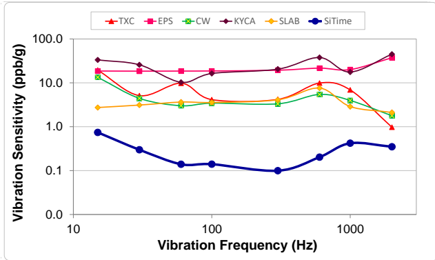
Figure 19. Vibration Robustness [5]
