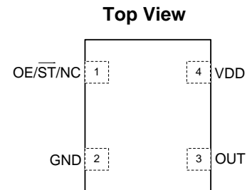
Figure 1. Pin Assignments
