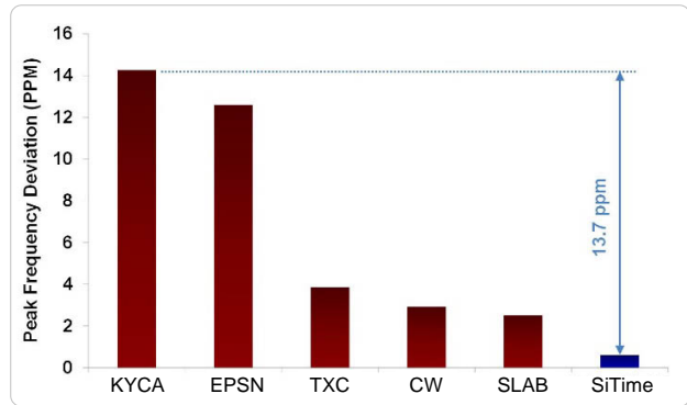
Figure 20. Shock Robustness [6]
