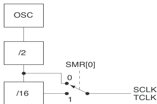
Figure 33. SCLK/TCLK Circuit
