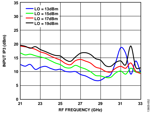
Figure 54. Input IP3 vs. RF Frequency at Various LO Powers, T A = 25°C
