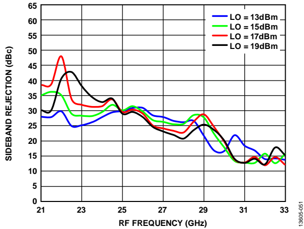
Figure 53. Sideband Rejection vs. RF Frequency at Various LO Powers, T A = 25°C
