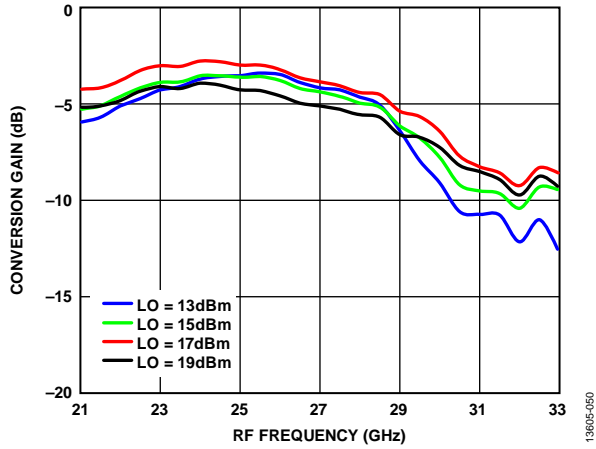
Figure 52. Conversion Gain vs. RF Frequency at Various LO Powers T A = 25°C
