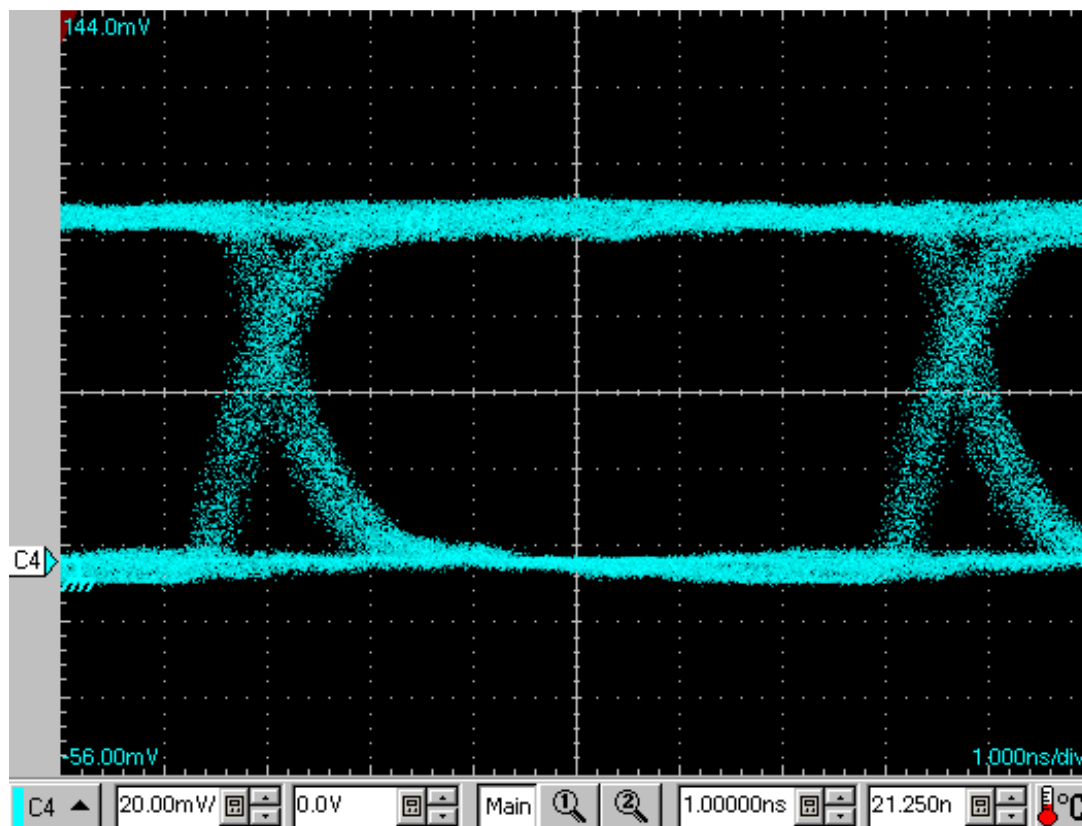
Figure 6. Eye Diagram
