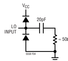
Figure 4. Equivalent Circuit Schematic of the LO Input
