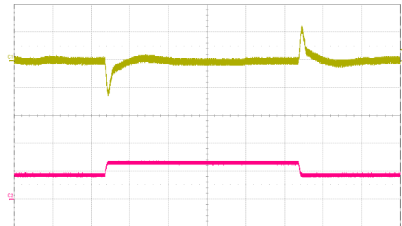
Fig. 12: Output voltage response to load current step change (18A – 27A – 18A) at V_{in} = 48\text{ V} . Top trace: output voltage (200 mV/div.). Bottom trace: load current (20 A/div.). Current slew rate: 1\ \text{A}/\mu\text{s} . C_o = 1\ \mu\text{F} ceramic + 10,000\ \mu\text{F} + 10\ \mu\text{F} tantalum. Time scale: 200 \mu\text{s}/\text{div} .
