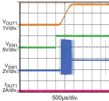
Enable On without Load I_{OUT1} = I_{OUT2} = 0A
