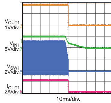
V_{IN} Power Down with 2A Load I_{OUT1} = 2A , I_{OUT2} = 0A
