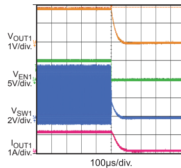
Enable Down with 2A Load I_{OUT1} = 2A , I_{OUT2} = 0A
