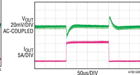
FIGURE 46 CIRCUIT V_{\text{IN}}=S_{\text{VIN}}=12\text{V} , V_{\text{OUT}}=1.2\text{V} , f_{\text{S}}=425\text{kHz} C_{\text{OUT}} = 3 \times 470\mu\text{F} POSCAP + 3 \times 100\mu\text{F} CERAMIC CAP \text{CCOMP}_{\text{b}}=47\text{pF} , \text{CCOMP}_{\text{a}}=2200\text{pF} R_{\text{TH}}=6 , g_{\text{m}}=4.36
