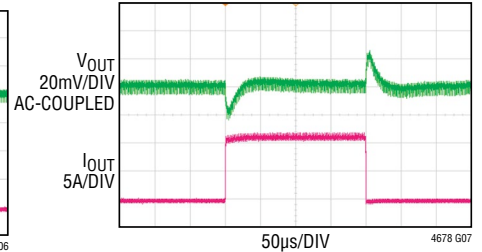
FIGURE 46 CIRCUIT V_{\text{IN}}=S_{\text{VIN}}=12\text{V} , V_{\text{OUT}}=1.5\text{V} , f_{\text{S}}=425\text{kHz} C_{\text{OUT}} = 3 \times 470\mu\text{F} POSCAP + 3 \times 100\mu\text{F} CERAMIC CAP \text{CCOMP}_{\text{b}}=47\text{pF} , \text{CCOMP}_{\text{a}}=2200\text{pF} R_{\text{TH}}=6 , g_{\text{m}}=4.36
