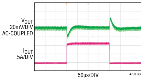
FIGURE 46 CIRCUIT V_{\text{IN}}=S_{\text{VIN}}=12\text{V} , V_{\text{OUT}}=1.8\text{V} , f_{\text{S}}=500\text{kHz} C_{\text{OUT}} = 3 \times 470\mu\text{F} POSCAP + 3 \times 100\mu\text{F} CERAMIC CAP \text{CCOMP}_{\text{b}}=47\text{pF} , \text{CCOMP}_{\text{a}}=2200\text{pF} R_{\text{TH}}=6 , g_{\text{m}}=4.36
