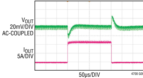
FIGURE 46 CIRCUIT V_{\text{IN}}=S_{\text{VIN}}=12\text{V} , V_{\text{OUT}}=1\text{V} , f_{\text{S}}=350\text{kHz} C_{\text{OUT}} = 3 \times 470\mu\text{F} POSCAP + 3 \times 100\mu\text{F} CERAMIC CAP \text{CCOMP}_{\text{b}}=47\text{pF} , \text{CCOMP}_{\text{a}}=2200\text{pF} R_{\text{TH}}=6 , g_{\text{m}}=4.36
