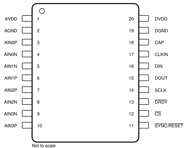
Figure 5-2. PW Package, 20-Pin TSSOP, Top View
