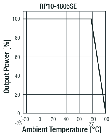
Derating Graph (11)
