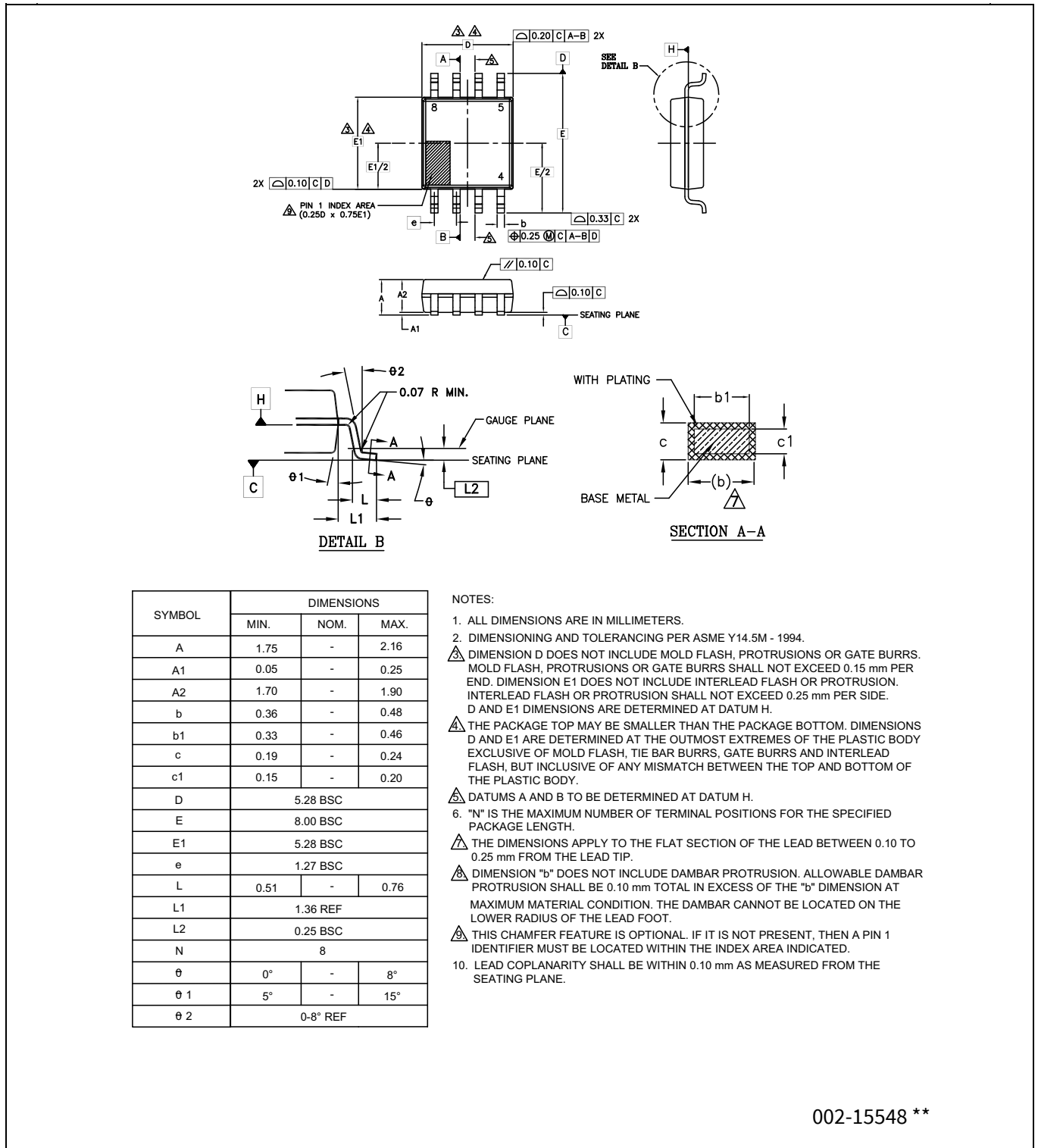
Figure 151 8-lead SOIC (5.28 × 5.28 × 2.16 mm) package outline (PG-DSO-8), 002-15548
