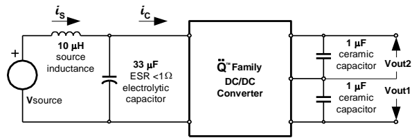
Figure 28. Test setup for measuring input reflected ripple currents, ic and is.
