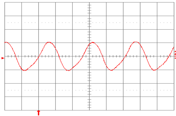
Figure 31. Input reflected ripple current, I_{ic} (100 mA/div), measured at input terminals at full rated load current on both outputs and V_{in} = 48\text{ V} . Refer to Fig. 30 for test setup. Time scale: 1\text{ }\mu\text{s/div} .
