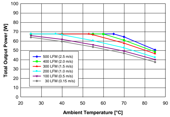
Figure 8. Available output power for balanced load current (Iout1 = Iout2) vs. ambient air temperature and airflow rates for converter mounted horizontally with Vin = 48 V, air flowing from pin 3 to pin 4 and maximum FET temperature ≤ 120 °C.
