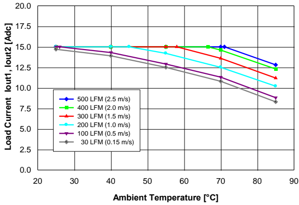
Figure 9. Available balanced load current (Iout1 = Iout2) vs. ambient air temperature and airflow rates for converter mounted vertically with Vin = 48 V, air flowing from pin 3 to pin 1 and maximum FET temperature ≤ 120 °C.
