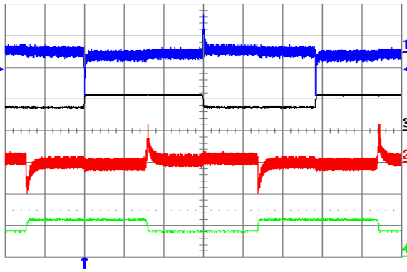
Figure 23. Output voltage response to both Iout1 and Iout2 (out of phase) load current step-change of 3.75 A (50%-75%-50%) at Vin = 48 V. Ch1 = Vout1 (50 mV/div), Ch2 = Vout2 (50 mV/div), Ch3 = Iout1 (10 A/div.), Ch4 = Iout2 (10 A/div.). Current slew rate: 0.1 A/μs, Co = 10 μF tantalum + 1 μF ceramic. Time scale: 1.0 ms/div.
