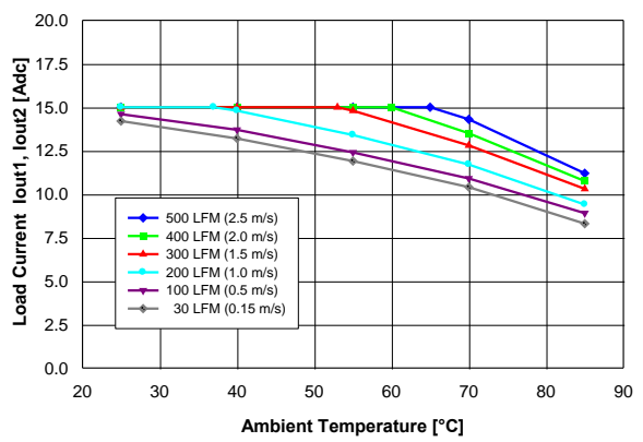
Figure 10. Available balanced load current (Iout1 = Iout2) vs. ambient air temperature and airflow rates for converter mounted horizontally with Vin = 48 V, air flowing from pin 3 to pin 4 and maximum FET temperature ≤ 120 °C.
