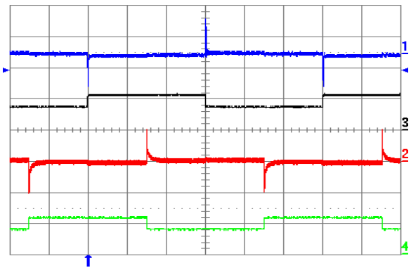
Figure 24. Output voltage response to both Iout1 and Iout2 (out of phase) load current step-change of 3.75 A (50%-75%-50%) at Vin = 48 V. Ch1 = Vout1 (100 mV/div), Ch2 = Vout2 (100 mV/div), Ch3 = Iout1 (10 A/div.), Ch4 = Iout2 (10 A/div.). Current slew rate: 5 A/μs, Co = 300 μF tantalum + 1 μF ceramic. Time scale: 1.0 ms/div.
