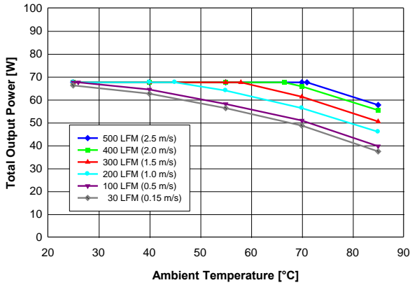
Figure 7. Available output power for balanced load current (Iout1 = Iout2) vs. ambient air temperature and airflow rates for converter mounted vertically with Vin = 48 V, air flowing from pin 3 to pin 1 and maximum FET temperature ≤ 120 °C.
