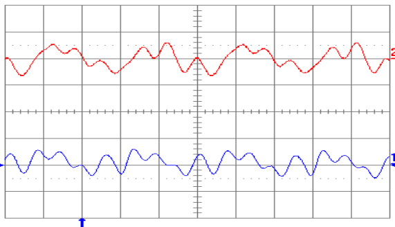
Figure 27. Output voltage ripple at full rated load current into a resistive load on both outputs with Co = 1μF (ceramic) and Vin = 48 V. Ch2 = Vout2, Ch1 = Vout1 (both 20 mV/div). Time scale: 1 μs/div.
