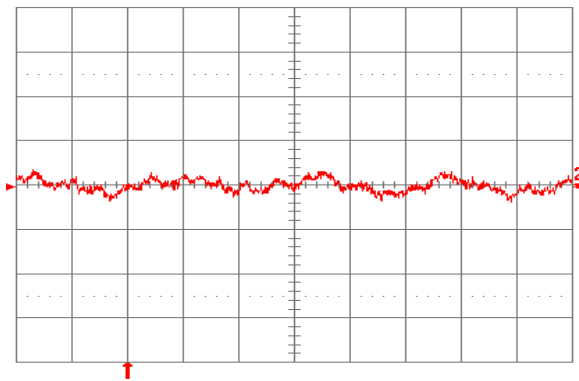
Figure 32. Input reflected ripple current, I_s (10 mA/div), measured through 10\text{ }\mu\text{H} at the source at full rated load current on both outputs and V_{in} = 48\text{ V} . Refer to Fig. 30 for test setup. Time scale: 1\text{ }\mu\text{s/div} .
