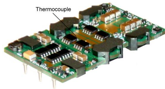
Figure 33. Location of the thermocouple for thermal testing.
