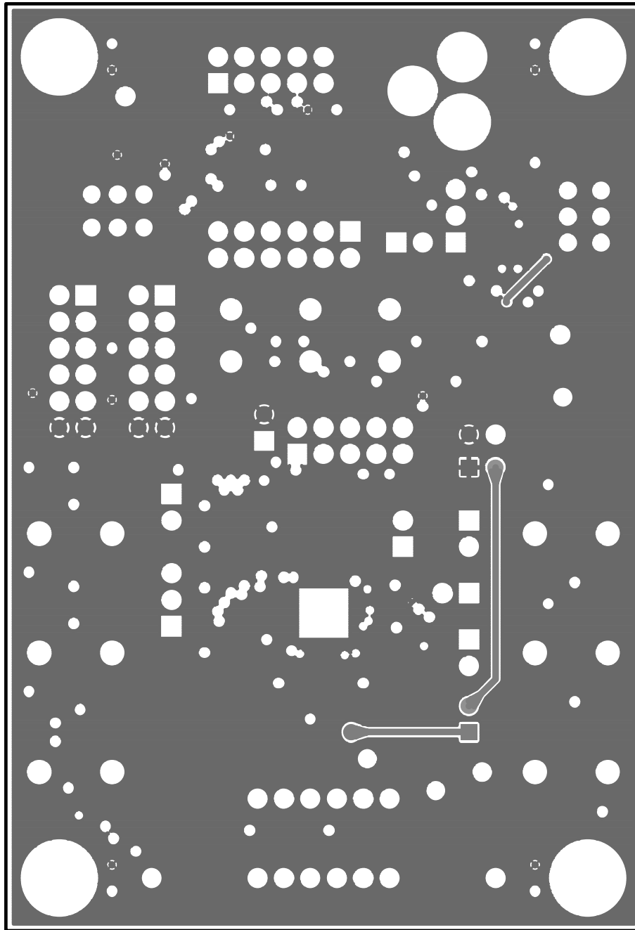
Figure 58. EVAL-ADAU1772Z Evaluation Board Layout—Power Plane
