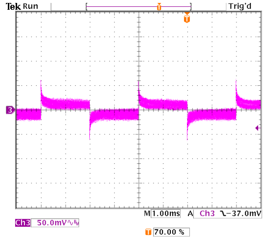
Figure 53. Transient Response with Regulation set to 0.74 mV/A.
