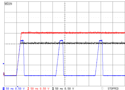
Figure 41. Turn-On into UVP on V3. The UV Fault Is Programmed To Be Non-Latching. Ch1 – Vo1, Ch2 – Vo2(Group A), Ch3 – Vo3 (Group B) Vo4 not shown.
