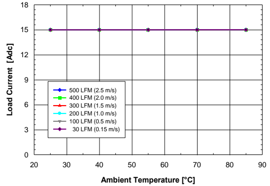
Figure 4. Available output current vs. ambient air temperature and airflow rates for converter DP7120G mounted horizontally with air flowing from input to output, MOSFET temperature \leq 120^{\circ}\text{C} , V_{in} = 12\text{ V} , V_{out} = 5\text{ V} , and F_{sw} = 1\text{MHz}
