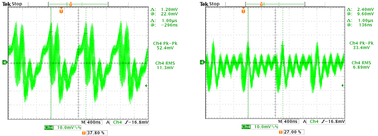
Figure 48. Input Voltage Noise with Interleave
