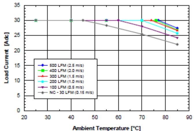
Fig. 1.5V.2: Available load current vs. ambient air temperature and airflow rates for SQE48T30015 converter mounted horizontally with air flowing from pin 3 to pin 1, MOSFET temperature \leq 120 ^{\circ} C, V_{in} = 48 V.
