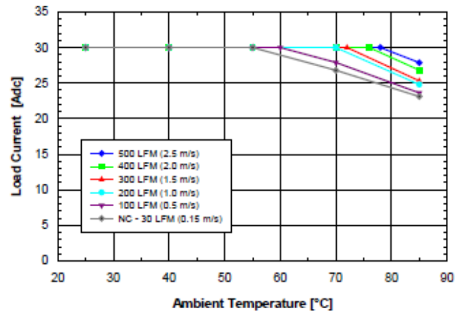
Fig. 1.5V.1: Available load current vs. ambient air temperature and airflow rates for SQE48T30015 converter mounted vertically with air flowing from pin 3 to pin 1, MOSFET temperature \leq 120 ^{\circ} C, V_{in} = 48 V.
