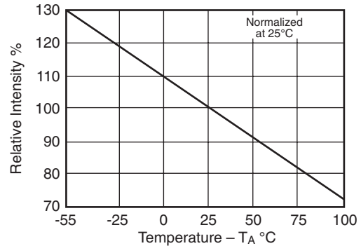
Fig. 4 Relative Luminous Intensity vs. Temperature
