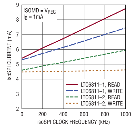
isoSPI Current (ACTIVE) vs isoSPI Clock Frequency
