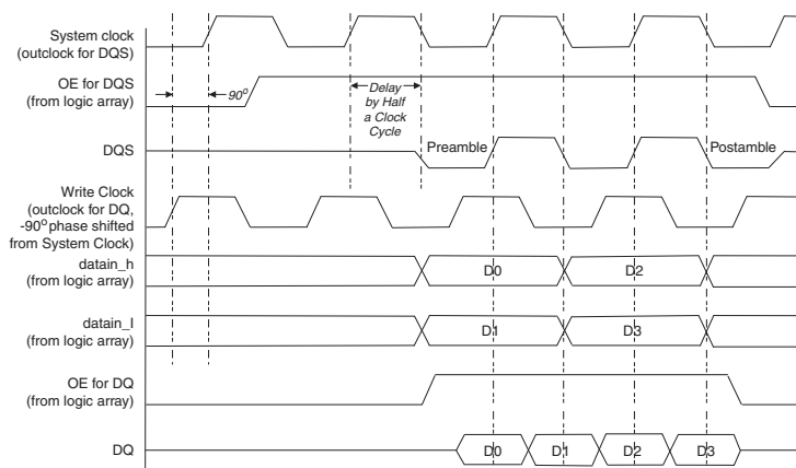
(1) The waveform reflects the software simulation result. The \overline{OE} signal is an active low on the device. However, the Quartus II software implements the signal as an active high and automatically adds an inverter before the A_{OE} register D input.
