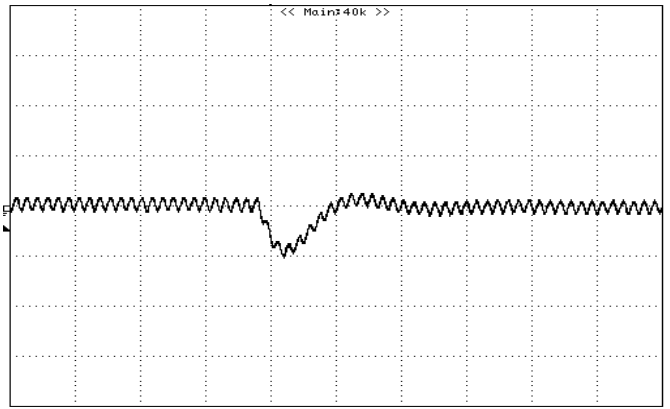
Figure 16: Typical transient response to step load change at 2.5A/\mu S from 50% to 100% of I_o , max at 12Vin, 5.0V out ( C_{out} = 1\mu F ceramic, 10\mu F tantalum) (200mV/div, 20uS/div)
