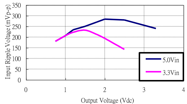
Figure 32: Input voltage ripple for various output models, I_O = 10 \text{ A} ( C_{IN} = 2 \times 100 \mu\text{F} tantalum // 47 \mu\text{F} ceramic)
