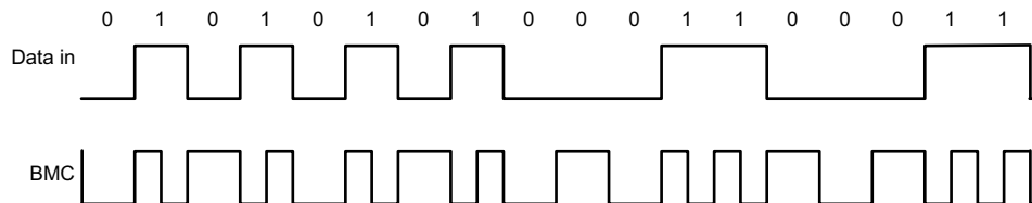
Figure 9-6. Biphasic Mark Coding Example
