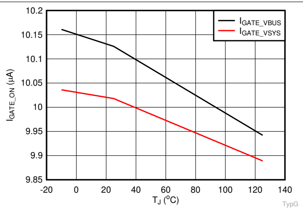
Figure 7-8. I GATE_VSYS_ON vs. Temperature for TPS25750S
