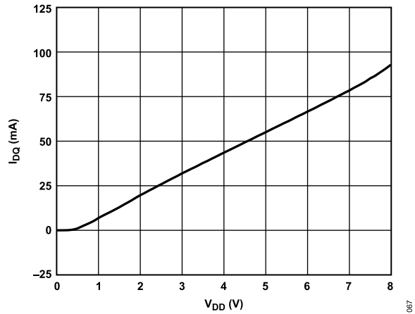
Figure 68. I_{DQ} vs. V_{DD} , Representative of a Typical Device, R_{BIAS} = 1.1 \text{ k}\Omega
