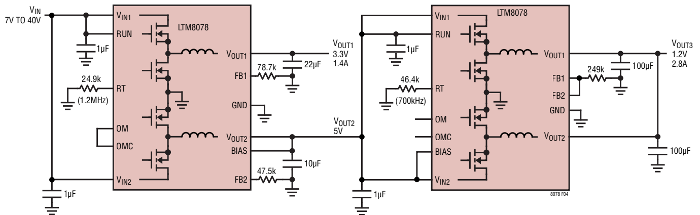
Figure 4. Cascade Two LTM8078 to Produce 3.3V, 1.4A, 1.2V, 2.8A from 7V to 40V IN , Both BIAS Pins Are Connected to V OUT2
