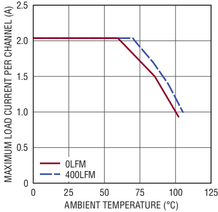
Derating, V_{IN} = 24\text{V} , V_{OUT} = 1.5\text{V} BIAS = 5V, DC2777A Demo Board Both Channels at Same Load
