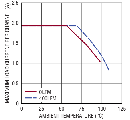
Derating, V_{IN} = 36\text{V} , V_{OUT} = 3.3\text{V} BIAS = 5V, DC2777A Demo Board Both Channels at Same Load
