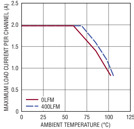
Derating, V_{IN} = 36\text{V} , V_{OUT} = 1.5\text{V} BIAS = 5V, DC2777A Demo Board Both Channels at Same Load
