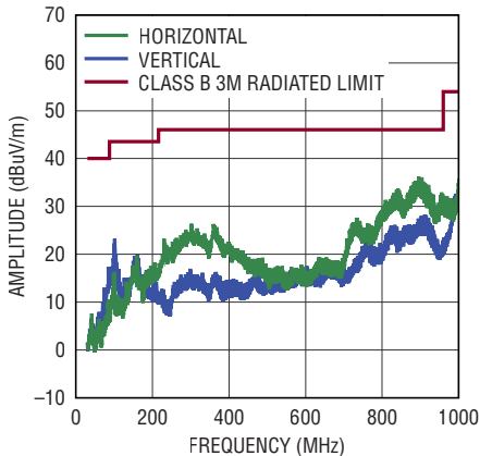
CISPR22 Class B Emissions 24\text{V}_{IN} , f_{SW} = 1.6\text{MHz} 5\text{V}_{OUT1} at 1.4A, 3.3\text{V}_{OUT2} at 1.4A Spread Spectrum On, No EMI Filter
