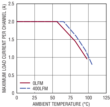
Derating, V_{IN} = 24\text{V} , V_{OUT} = 3.3\text{V} BIAS = 5V, DC2777A Demo Board Both Channels at Same Load
