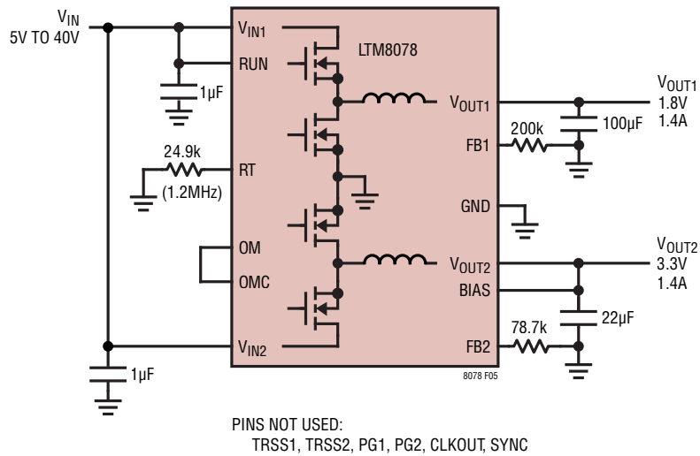
Figure 5. 1.8V, 1.4A and 3.3V, 1.4A from 5V to 40V IN , BIAS Is Connected to V OUT2
