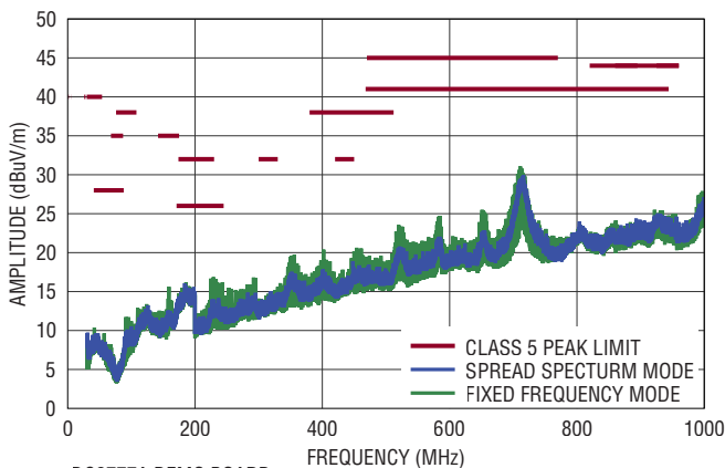
DC2777A DEMO BOARD V_{IN} = 12\text{V} , V_{OUT} = 3.3\text{V} TWO CHANNELS PARALLELED, I_{OUT} = 2.8\text{A} , f_{SW} = 1\text{MHz}
