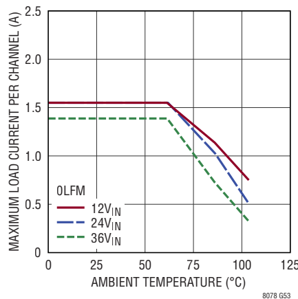
Derating, V_{OUT} = 10\text{V} , BIAS = 5V, DC2777A Demo Board Both Channels at Same Load
