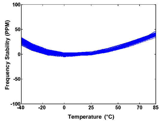
Figure 6. Frequency Stability Over Temperature
