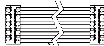
BROWN WIRE INDICATES PIN #1 STANDARD WIRING
