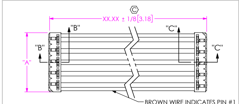
FIG 2 IDSS-05-S-XX.XX-XXX-XXX SHOWN (DIFFERENT AS SHOWN, OTHERWISE SAME AS FIG 1)
