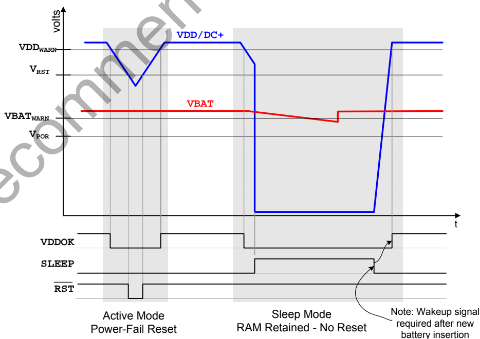
Figure 18.3. Power-Fail Reset Timing Diagram
