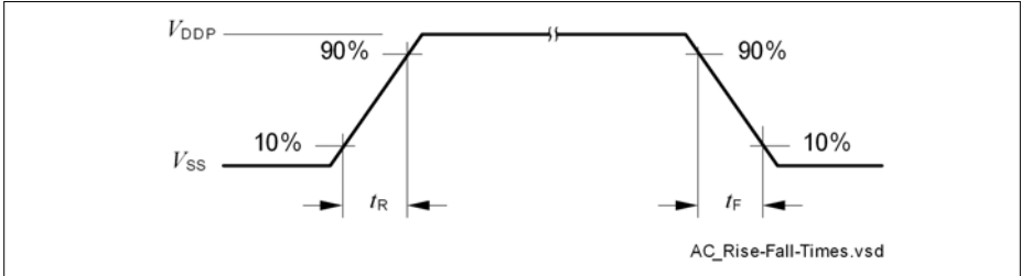
Figure 23 Rise/Fall Time Parameters
