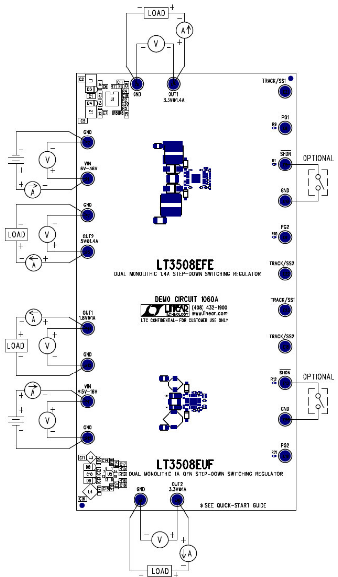
Figure 3. Proper Measurement Equipment Setup
