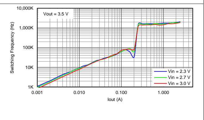
Figure 31. Switching Frequency
