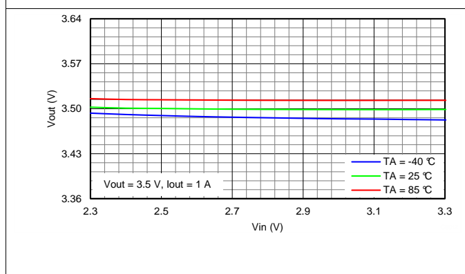
Figure 30. Line Regulation
