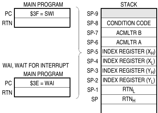
Figure 3-2. Stacking Operations
