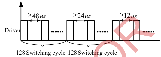
Figure 2— t_{\text{minoff}} at start-up Constant Voltage (CV) Operation
