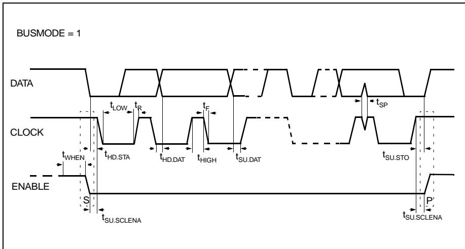
Figure 8 3-Wire Bus
