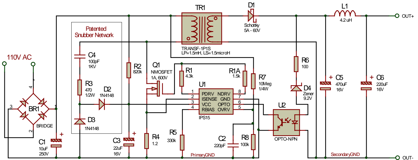
TYPICAL APPLICATION SCHEMATIC: AC IN 110V, 5W OUTPUT, zener regulation (EMC components not shown).
