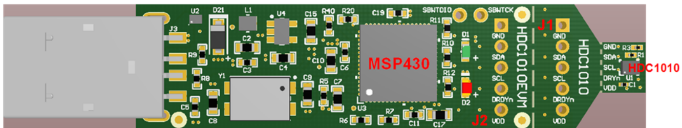
Figure 1. HDC1010EVM
