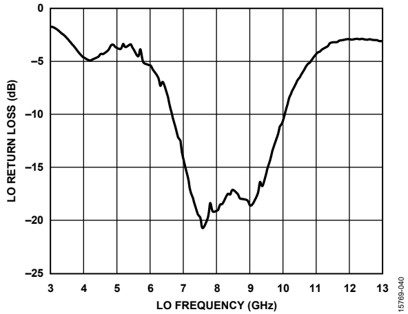
Figure 40. LO Return Loss vs. LO Frequency
