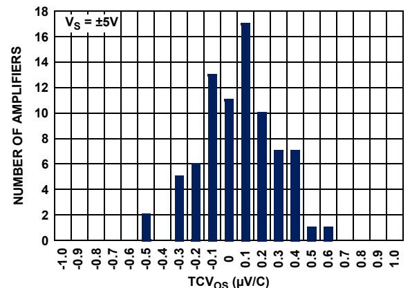
FIGURE 8. ISL28118 TCV 0S vs NUMBER OF AMPLIFIERS ±5V
