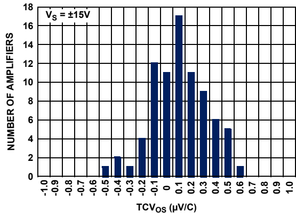
FIGURE 7. ISL28118 TCV 0S vs NUMBER OF AMPLIFIERS ±15V
