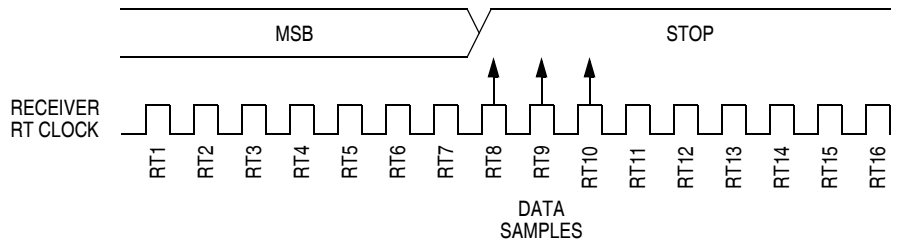
Figure 13-8. Slow Data
