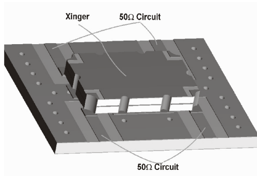
Figure 4: Component Placement
