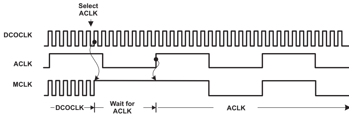
Figure 3-4. Switch MCLK From DCOCLK to LFXTCLK
