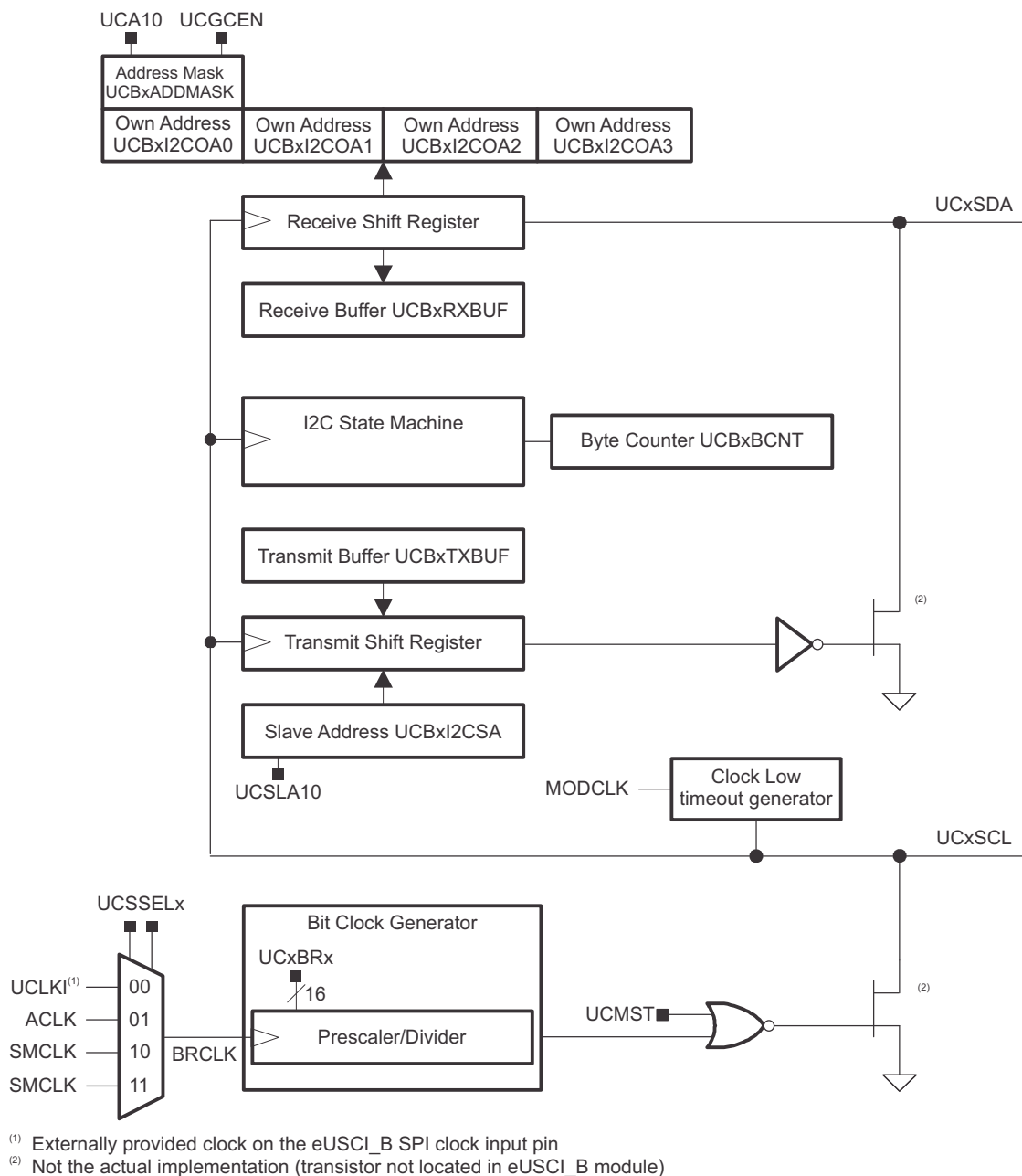
Figure 32-1. eUSCI_B Block Diagram – I 2 C Mode
