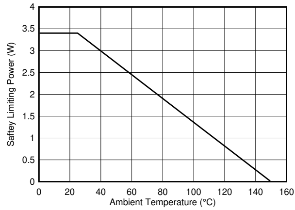
Figure 7-30. Thermal Derating Curve for Safety-Limiting Power
