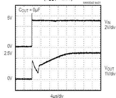
TURN-ON TRANSIENT ( V_{OUT} = 2.5V )
