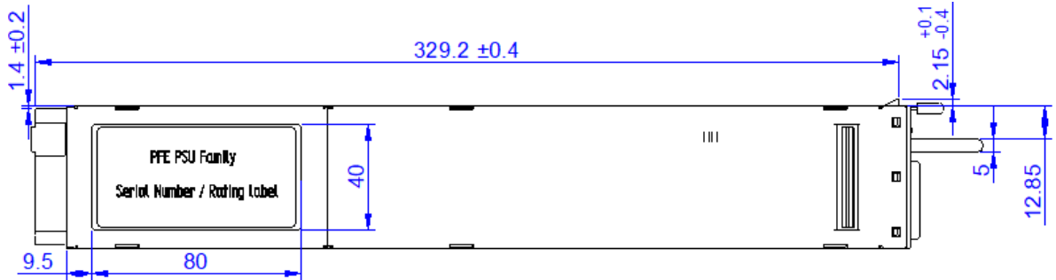
Figure 42. Top View
