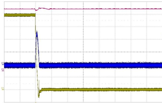
Figure 9. Short circuit on V1 (500 μs/div) CH1: V 1 (2 V/div) CH2: V SB (1 V/div) CH3: I 1 (200 A/div)
