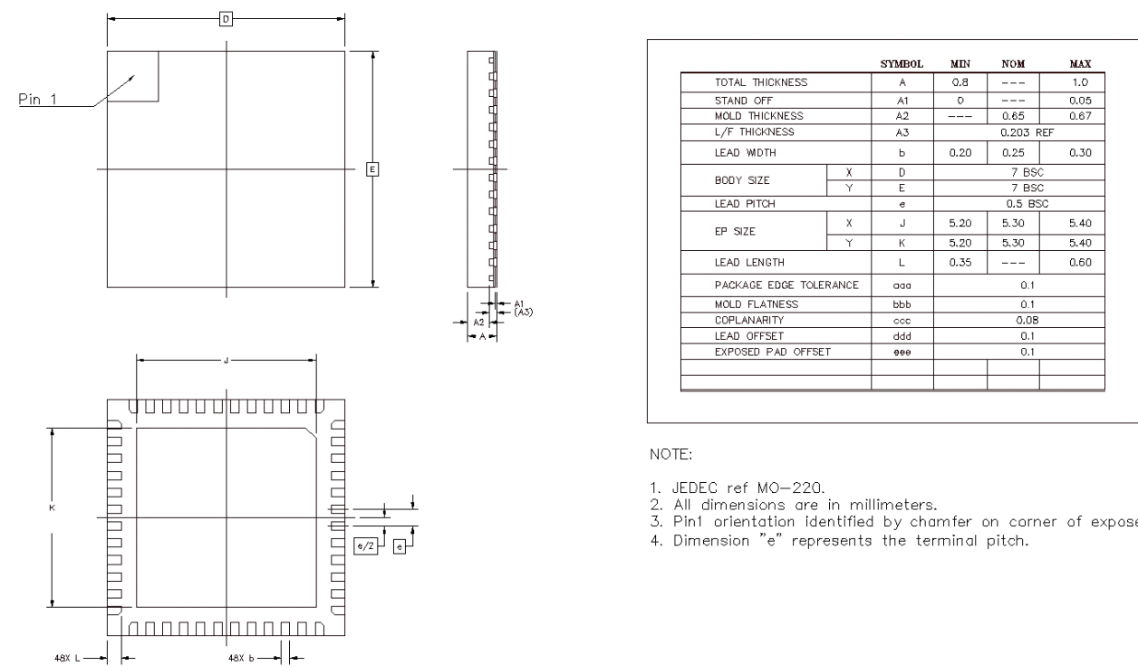
Figure 20.1. Package Drawing
