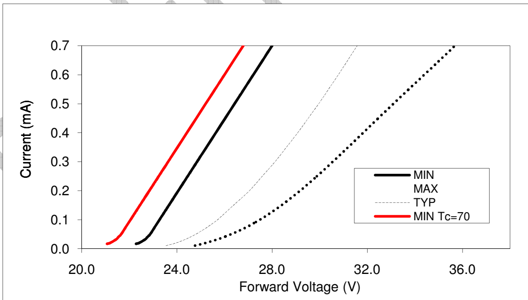
Figure 11: Typical Current vs. Voltage BXR-XXX0740-A, BXR-40E0810-A, BXRA-56C1000
