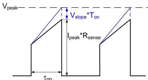
Typical Waveform
