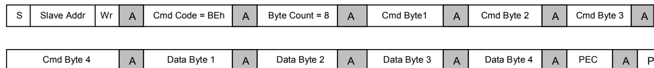
Figure 7-3 SMBus Block Write Command Format, to Write to a PI7C9X2G1616PR Register with PEC
