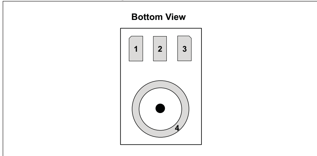
Figure 1. Pin connections
