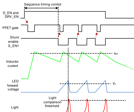
Figure 7-17. Discontinuous Mode Operation Inductor Current/LED Voltage
