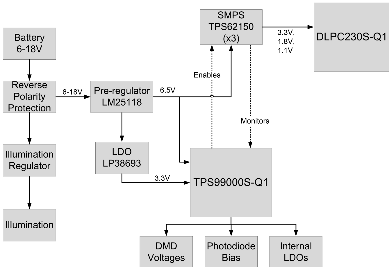
Figure 9-3. Architecture Number 3: Headlight Application with Independent Illumination
