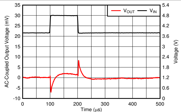
V_{\text{OUT}} = 3.3\text{ V} , I_{\text{OUT}} = 50\text{ mA} , slew rate = 1\text{ V}/\mu\text{s} , T_J = -40^\circ\text{C}
