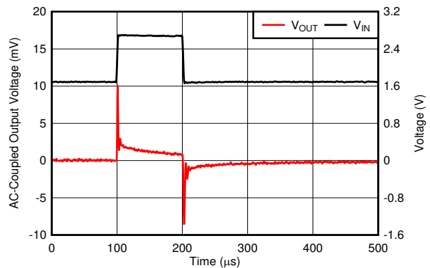
V_{\text{OUT}} = 1.2\text{ V} , I_{\text{OUT}} = 300\text{ mA} , slew rate = 1\text{ V}/\mu\text{s} , T_J = 150^\circ\text{C}
